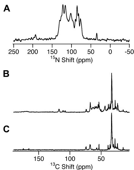
Fig. 7. One-dimensional spectra of various magnetically aligned bicelle samples. (A) 15 N NMR spectrum of uniformly 15 N labeled p7 protein from HCV in magnetically aligned bicelles. (B) 13 C NMR spectrum of partially 13 C-labeled Pf1 coat protein in magnetically aligned bicelles. (C) 13 C NMR spectrum of bicelles without protein; the comparison of (B) and (C) enables the protein resonances to be distinguished.
