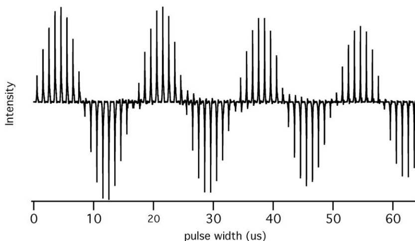
Fig. 5. ^1\text{H} nutation plot at 800 MHz for the water resonance in a typical bicelle sample in a 9 mm long and 5 mm OD sample tube. The nutation plot is obtained by measuring the resonance intensities following direct excitation with pulses of various durations.
