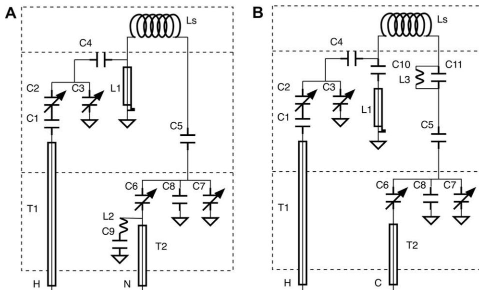
Fig. 3. (A) Circuit diagram of the ^1\text{H}/^{15}\text{N} double-resonance probe. (B) Circuit diagram of the ^1\text{H}/^{13}\text{C} double-resonance probe.
