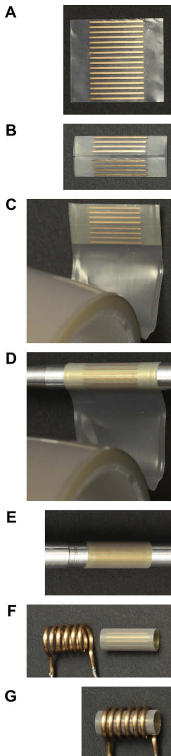
Fig. 1. Constructions of a strip-shield. (A) One strip-shield is cut from the larger PTFE sheet. (B) With the copper on the outside, the sheet is rolled to form a cylinder. (C) PTFE tape is applied to connect the ends. (D) The rolled sheet is placed on a 5 mm OD cylinder, and wrapped with two layers of PTFE tape. (E) Excess PTFE is cut off from both ends. (F) The strip-shield is inserted into a 5.6 mm ID solenoid coil. (G) The completed strip-shield/coil assembly.
