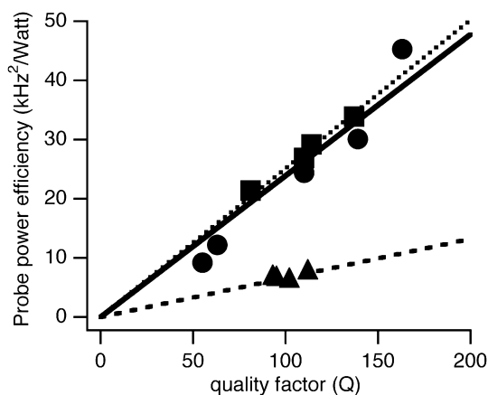
Fig. 4. Plots of probe power efficiency vs. the quality factor of the circuit. Circle: ^1\text{H} channel; Squares: ^{13}\text{C} channel; Triangles: ^{15}\text{N} channel.
