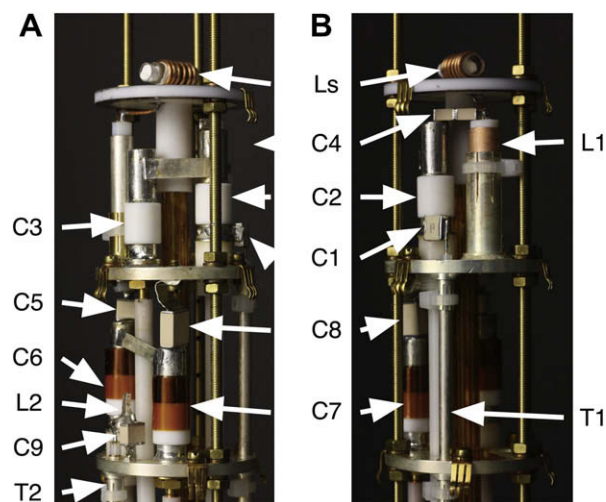
Fig. 2. Photographs of a ^1\text{H}/^{15}\text{N} double-resonance probe. (A and B) differ by 90° rotation. The inductors and capacitors are designated as in Fig. 3A and their values are listed in Table 1.
