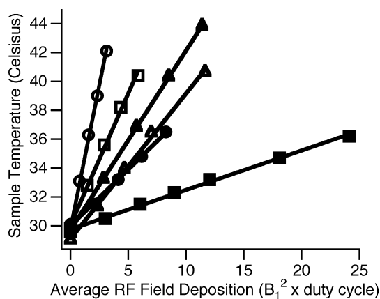
Fig. 6. Plots of measured sample temperature vs. RF Power Deposition. Open symbols: without shield; Filled symbols: with shield; Circles: 1 H channel; Squares: 13 C channel; Triangles: 15 N channel.
